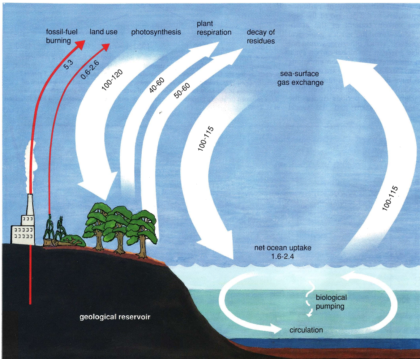
Figure 5. Massive flows between reservoirs make up the global carbon cycle. Plants on land take in carbon dioxide through photosynthesis. The terrestrial biosphere returns carbon to the atmosphere through plant respiration, the decomposition of plant residues and natural fires. The clearing of land for human activities also transfers carbon from the terrestrial system to the atmosphere. Meanwhile, gases are exchanged rapidly at the ocean surface; carbon is transferred to the deep ocean by circulation and by biological production (the use of carbon by surface organisms to produce compounds that enter the food chain of marine life). The ocean is believed to accumulate about two gigatons of carbon per year; most of this carbon is eventually dissolved in deep-ocean waters. Fossil-fuel burning transfers carbon from the geological reservoir to the atmosphere. All carbon fluxes are 1980 estimates, in gigatons.
