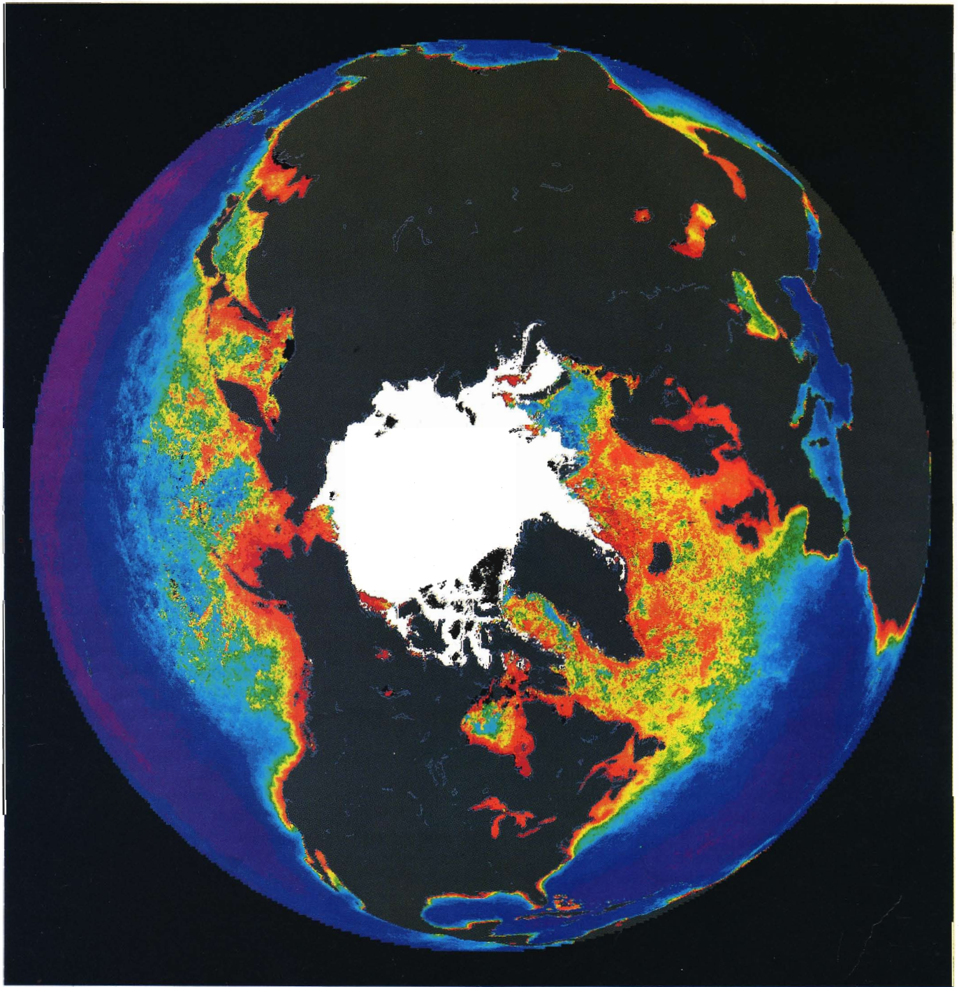
Figure 9. Polar oceans are the sites of abundant biological activity, as shown in these composite images produced by the Coastal Zone Color Scanner, which operated on the Nimbus-7 satellite from 1978 to 1986. Phytoplankton blooms in both the Arctic and Antarctic oceans are highly seasonal, limited by the availability of sunlight. The images are based on cumulative radiometric measurements of phytoplankton
