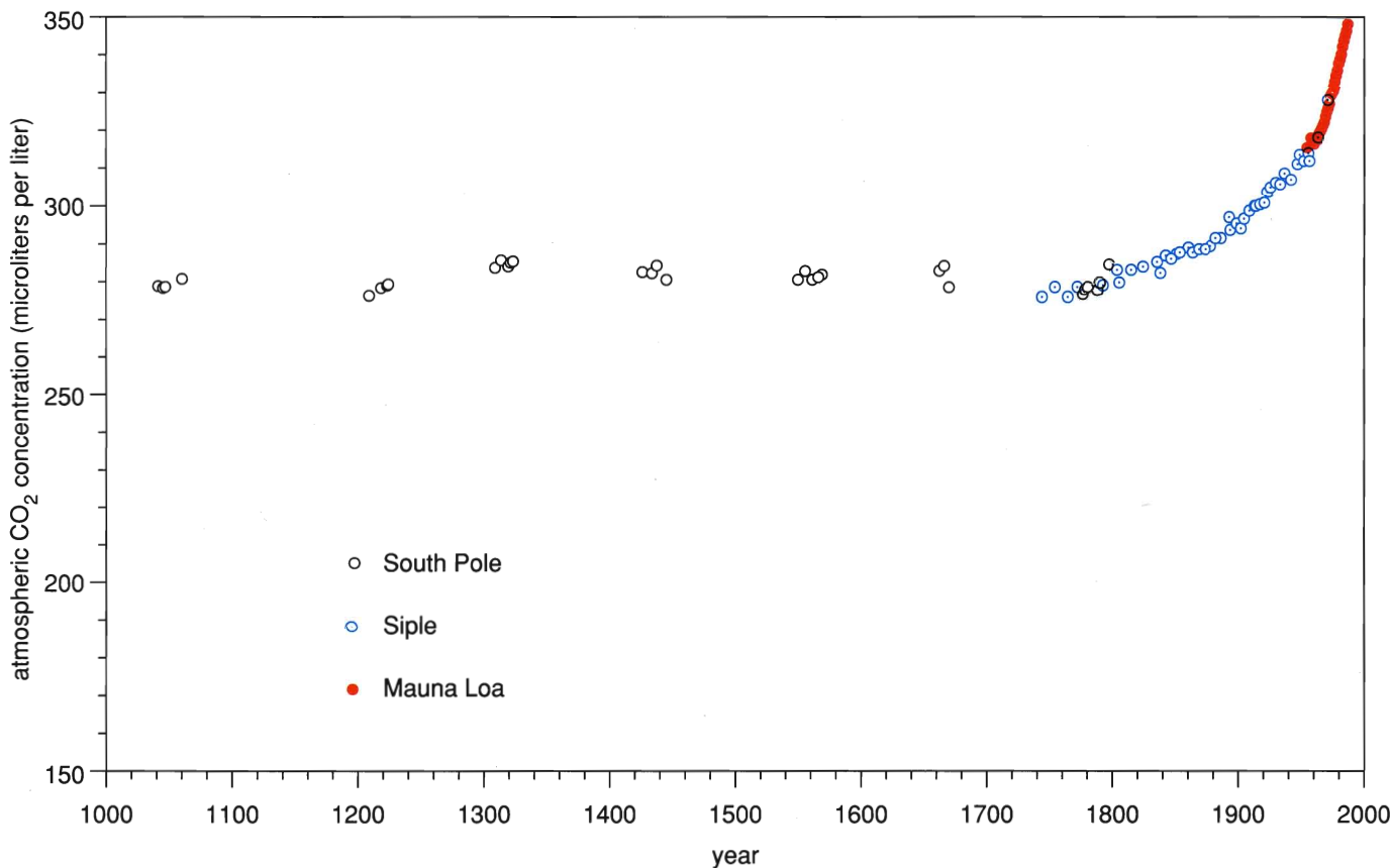
Figure 3b. Atmospheric CO 2 began increasing in the 18th century, and direct measurements made at Mauna Loa Observatory in Hawaii since 1958 indicate that the increase has accelerated. In 1988 the atmospheric carbon reservoir was estimated at 748 gigatons, equivalent to a CO 2 concentration of 351 microliters per liter and larger than at any time during the past 160,000 years. The South Pole and Siple ice-core data are from Neftel et al. 1985, Friedli et al. 1986 and Siegenthaler et al. 1988.
